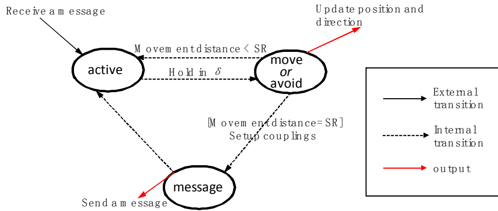
Fig. 2 Agent state transition diagram
