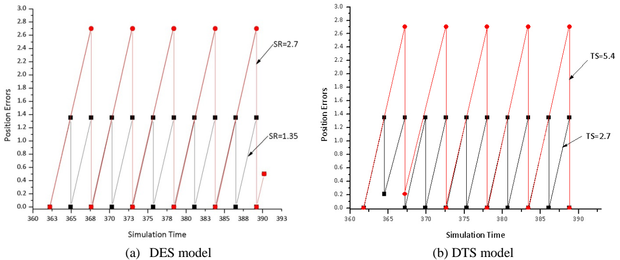
Fig. 6 Position errors in DES model and DTS model ( SR=1.35 and 2.7 , correspondingly TS = 2.7 and 5.4 )
