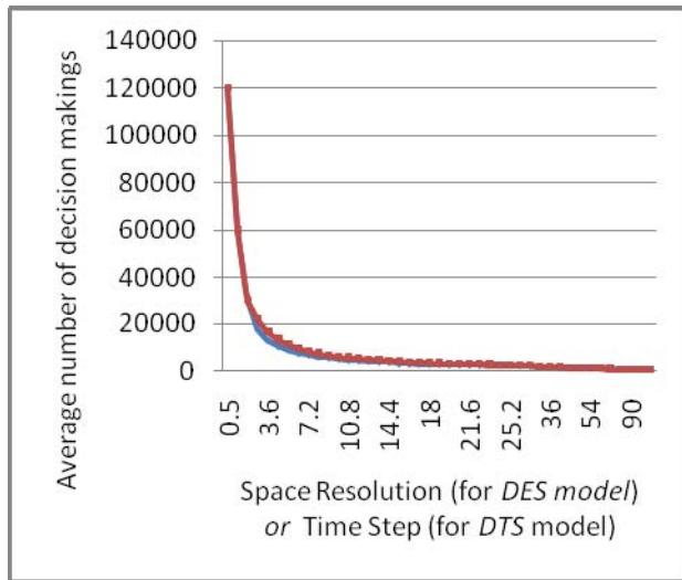
Fig. 8 SR/TS and decision makings (same speed)
