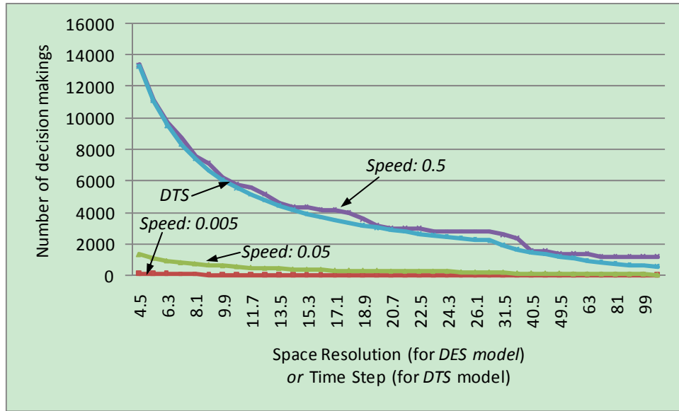
Fig. 10 SR/TS and individual agents' decision makings (different speed)
