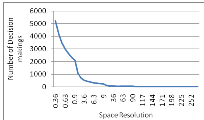
Fig. 7 Relationship between space resolution and number of decision makings of DES model
