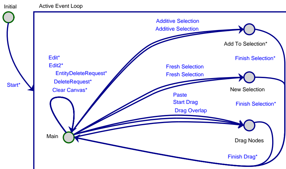
Figure 3.8: Post UI observer statechart
