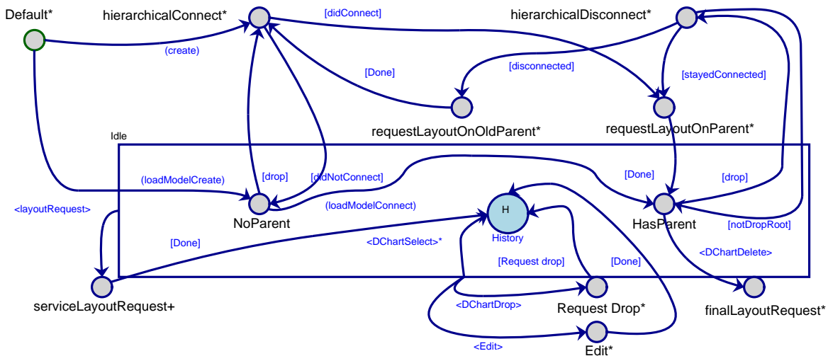
Figure 3.11: DC_Composite behaviour statechart
