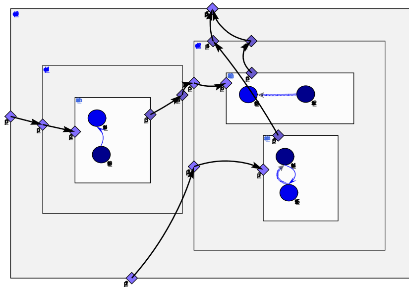
Figure 2.10: Sample model in the DEVS formalism
