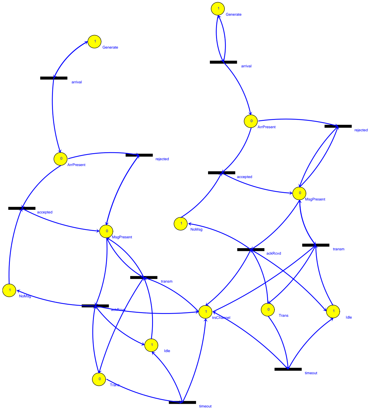
Figure 2.8: Transmitter model in the Petri Net formalism
