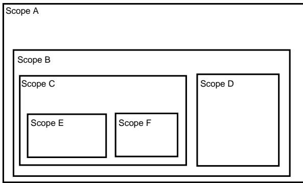
Figure 3.2: Hierarchical scopes
