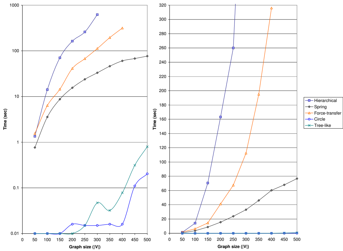
Figure 2.12: Time performance (logarithmic and normal time)
