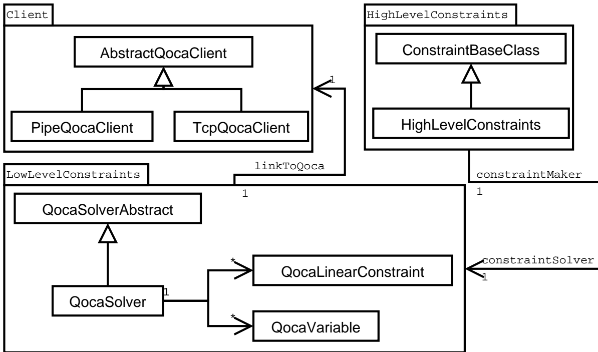
Figure 2.14: QOCA client class diagram
