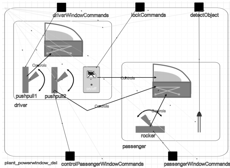
Fig. 6: Plant DSL: Example Model
