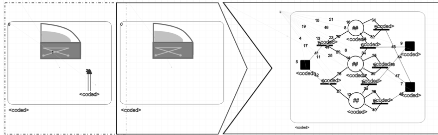
Fig. 8: Transformation Rule for Building a Petri Net Representation of a Power Window without Obstacle Sensor Plant
