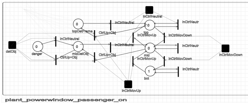
Fig. 7: Transformed Passenger Window Plant Model
