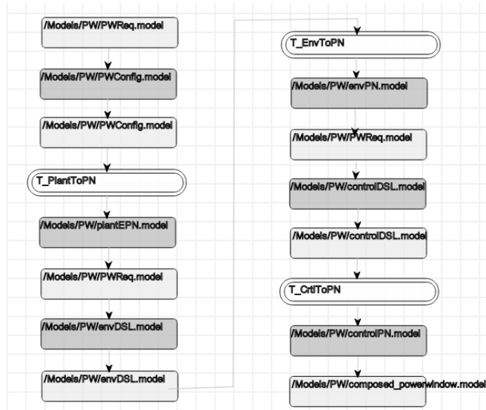
Fig. 4: The resulting transformation model of the example FTG+PM
