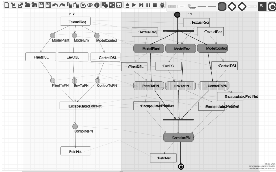
Fig. 1: Example FTG+PM Model
