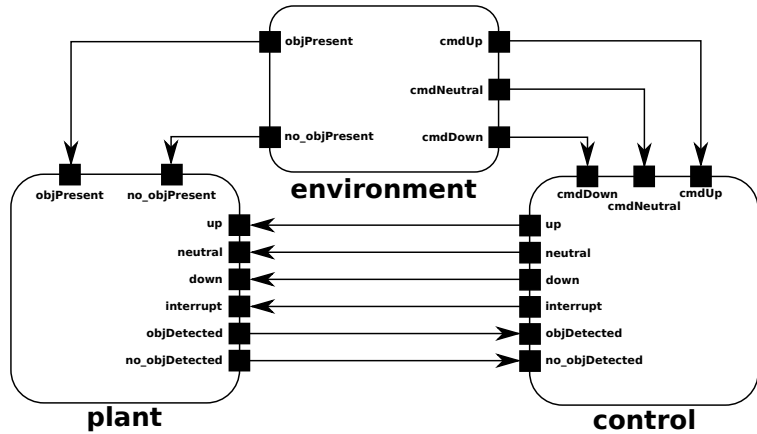
Figure 8: Architecture model.
